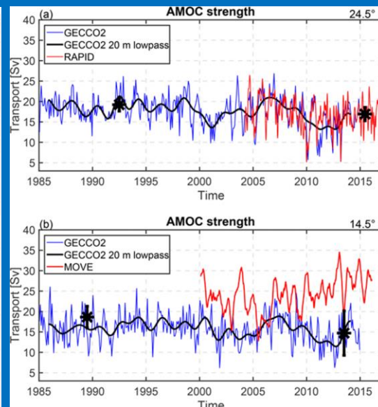
AMOC: Atlantic Meridional Overturning Circulation
