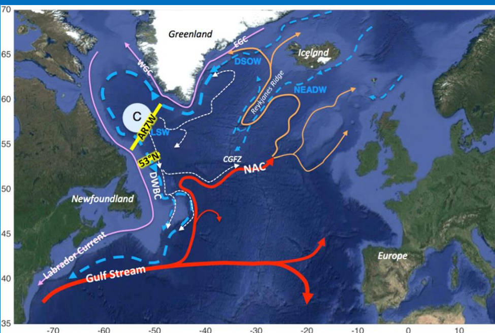
AMOC: Atlantic Meridional Overturning Circulation
